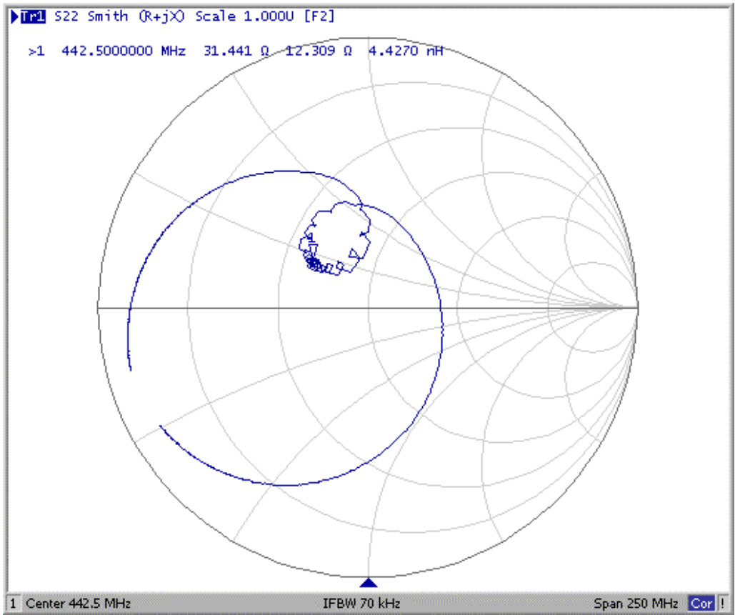
S22 Smith Chart:
