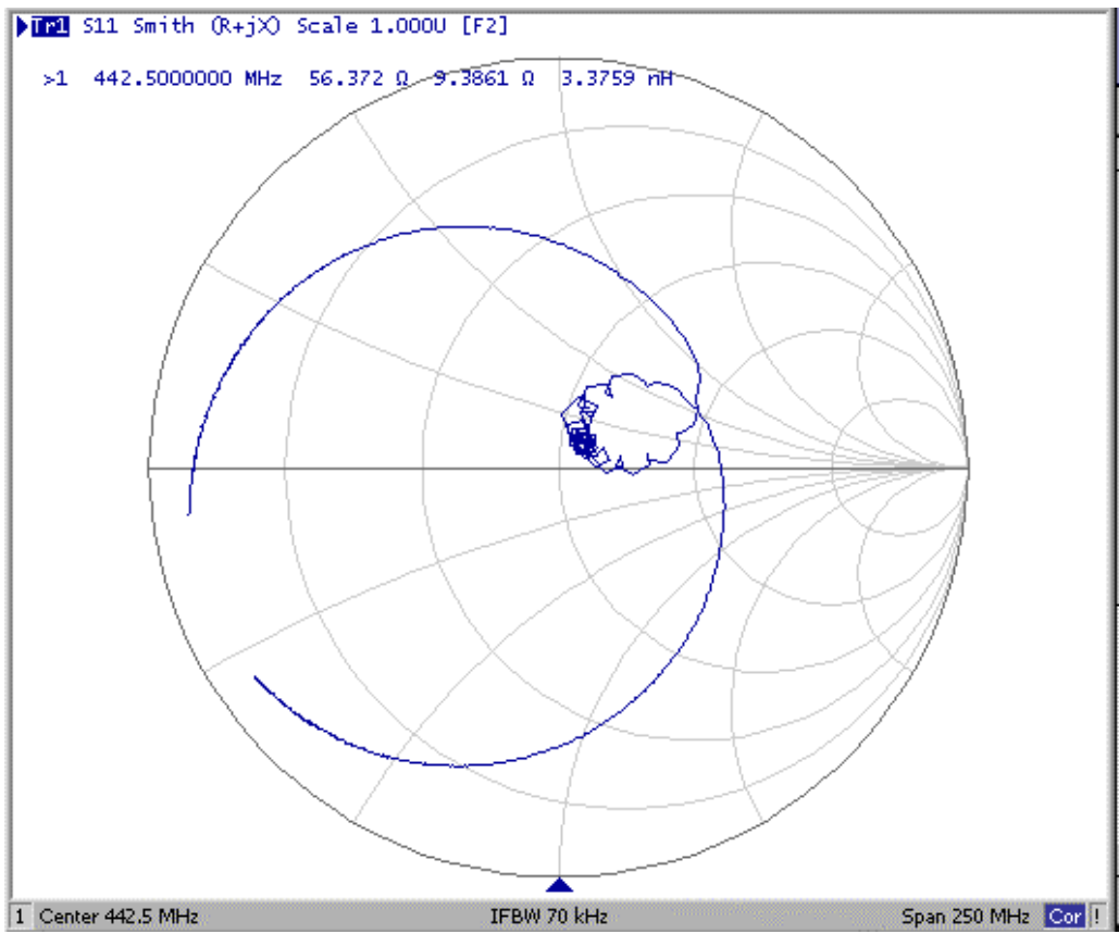
S11 Smith Chart:
